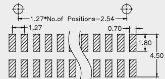
Recommended P.C.B Layout(Top Side)
